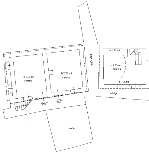
piano terreno
