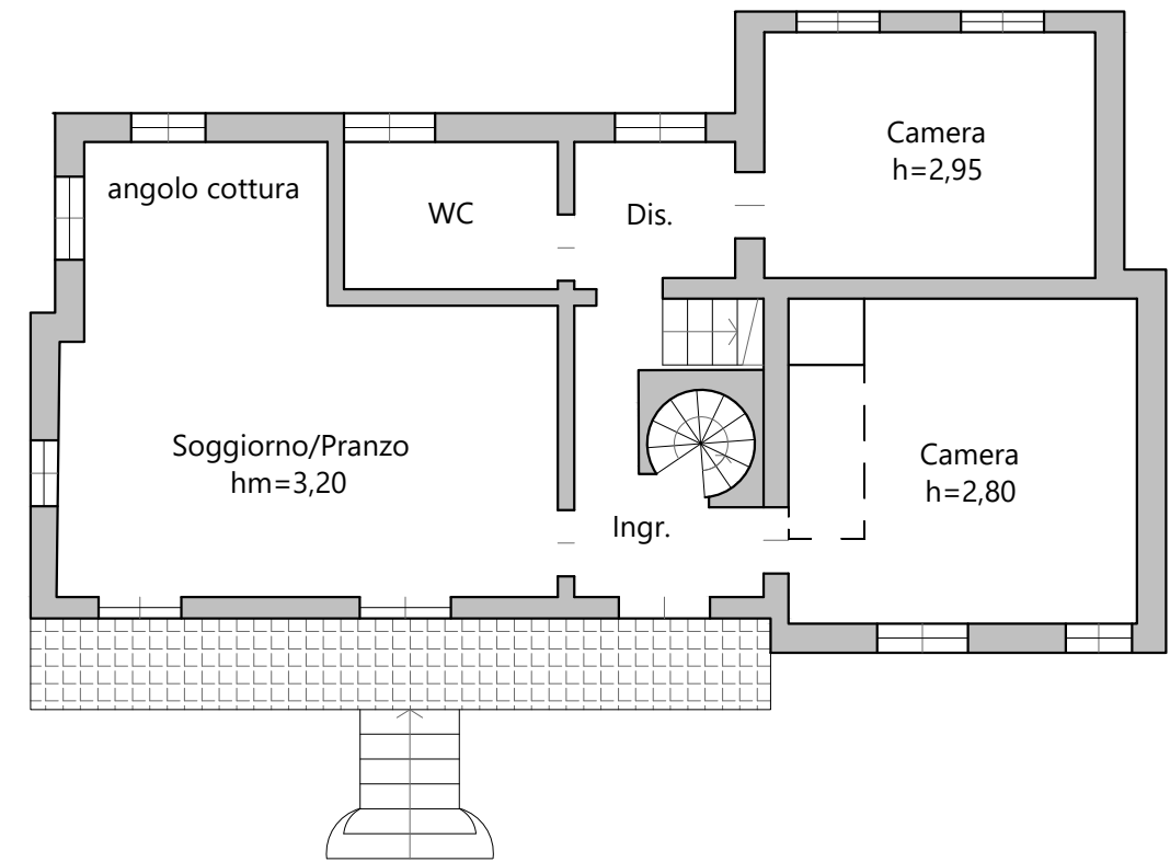
PIANO TERRA
